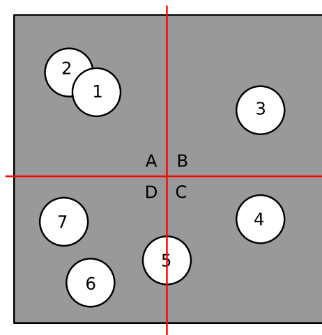
Figure 175: Graphical example of a quad tree, overlaid on the reference image
